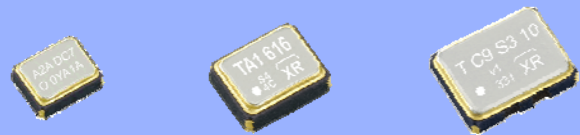
TG-5031CJ (2.0 × 1.6 × 0.73 mm) TG-5021CG (2.5 × 2.0 × 0.8 mm) TG-5021CE (3.2 × 2.5 × 0.9 mm)
